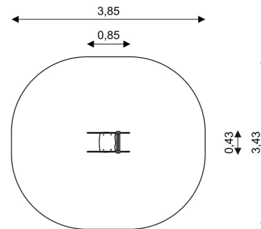
Minimal space
